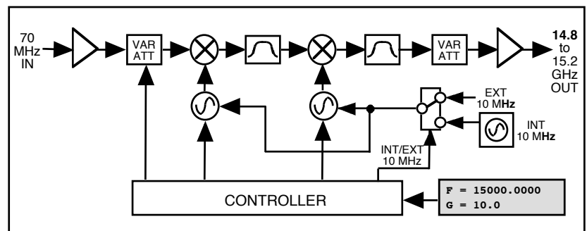
2015-152 Block Diagram
