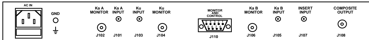
2584-31 Front and Rear Panels
